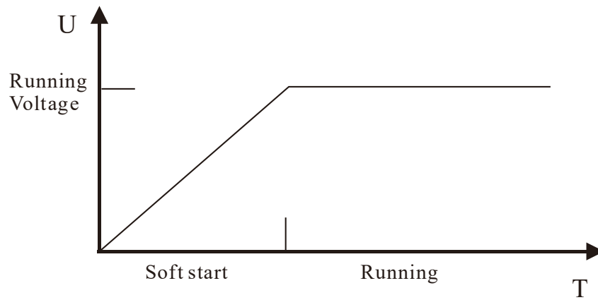
Soft Start Process Diagram
